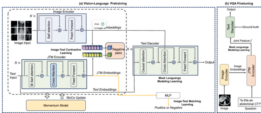
Fig. 9. Illustrate Pretraining (a) and Finetuning (b) of MISS framework [193].
