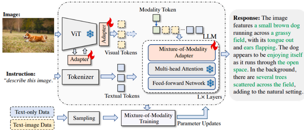
Fig. 10. Illustrate LaVIN framework (Multi-Modal Adapters) [203].
