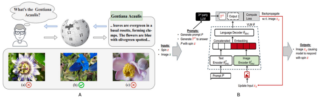
Fig. 8. Overview of prompt types in VLM: (A) Discrete prompts [78] and (B) Continuous prompts [102].
