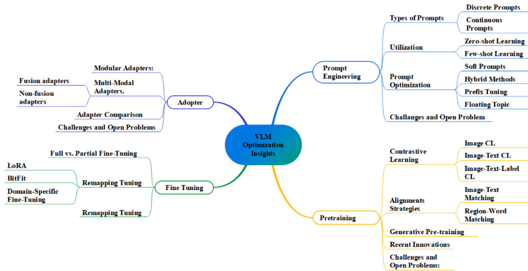
Fig. 2. Conceptual model of the paper.
